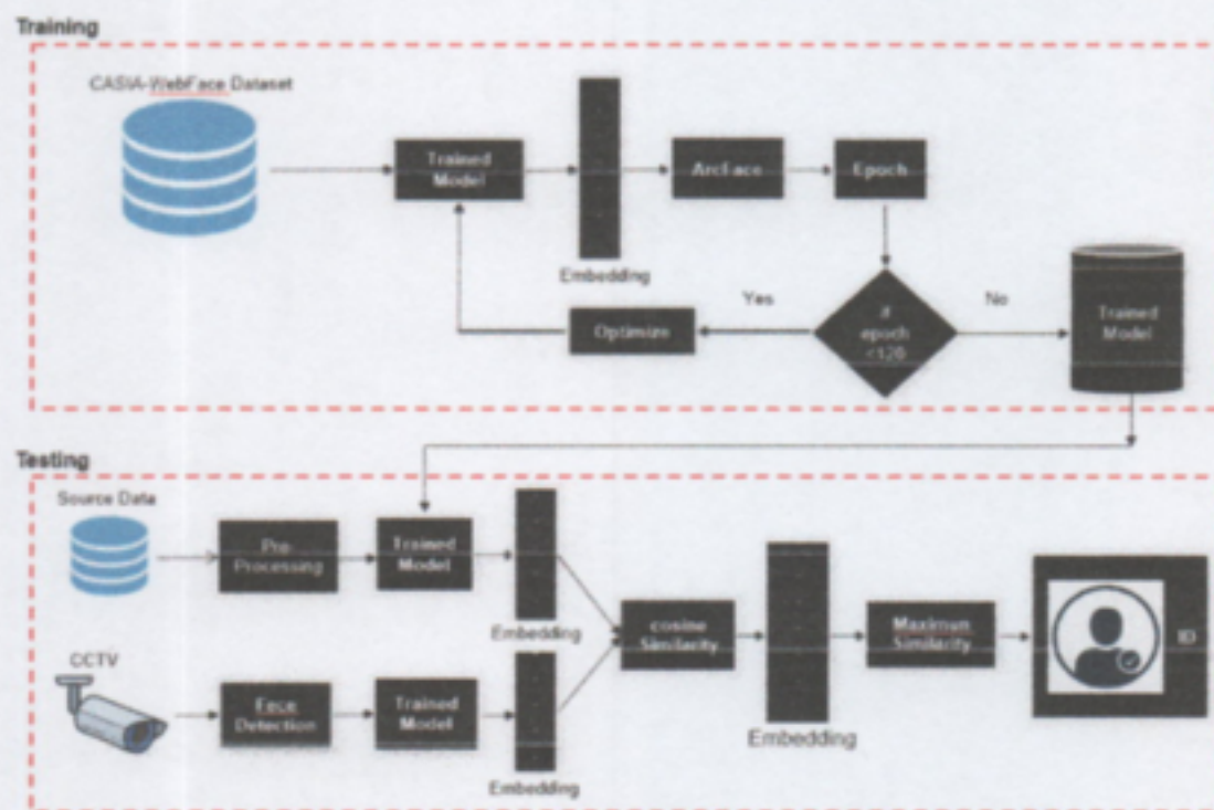
Figure 1. System Design
